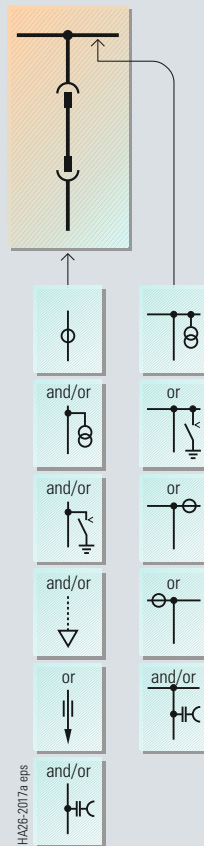
Disconnecting panel
